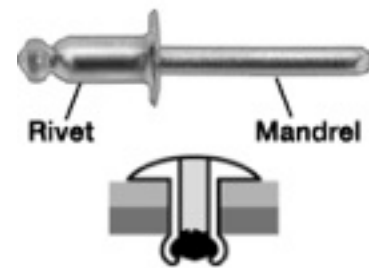
Fig 2b blind rivet
